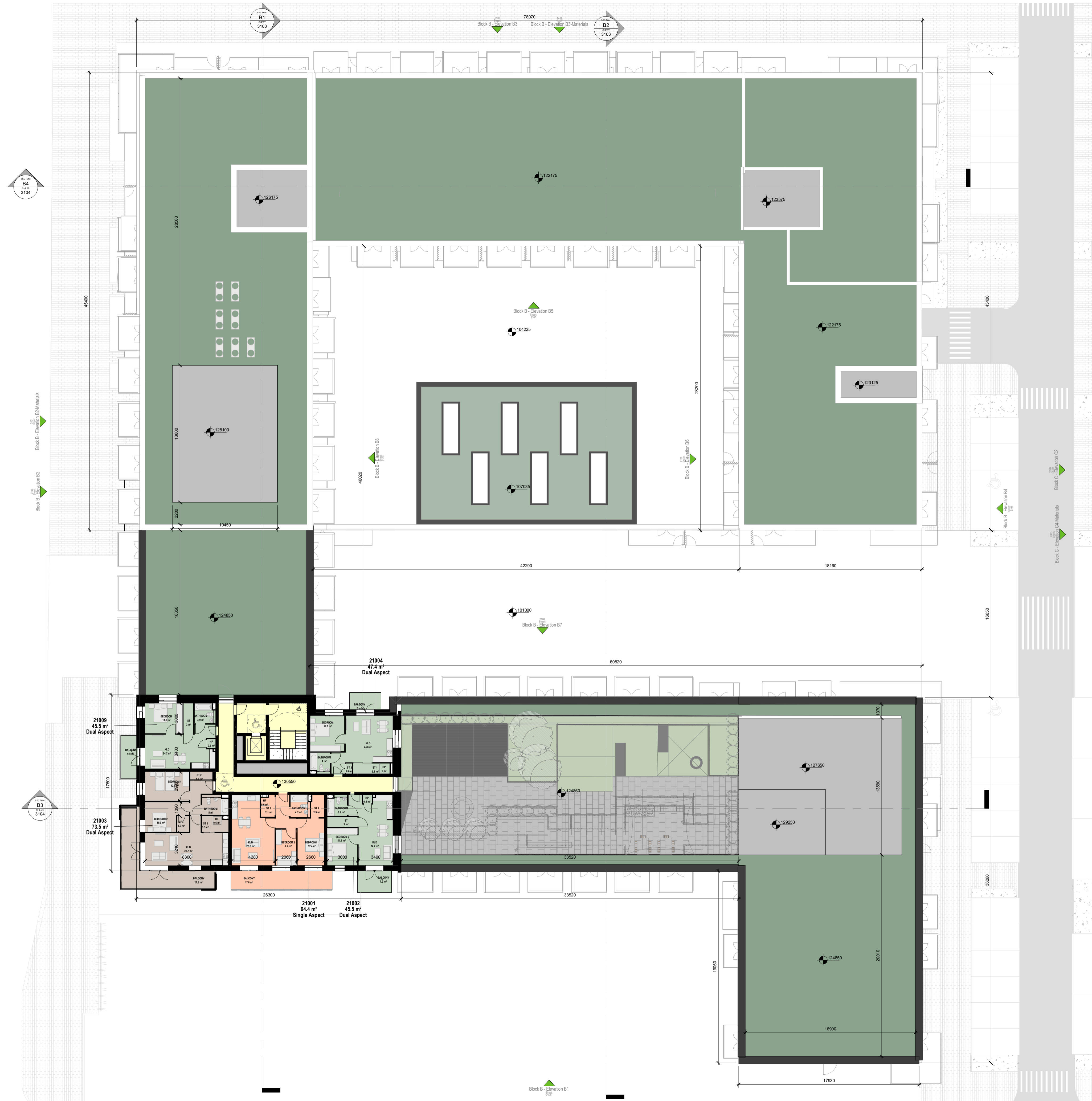
1 Plan - Block B - Level 10 1 : 200
